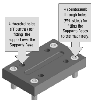
Supports Base art.BD LV...FPL with countersunk through holes at sides. Normally used for fixed supports with bearings and DVC with bush.
