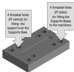
Supports Base art.BD LV...FF series with threaded holes. Normally used for mobile support with nut.
